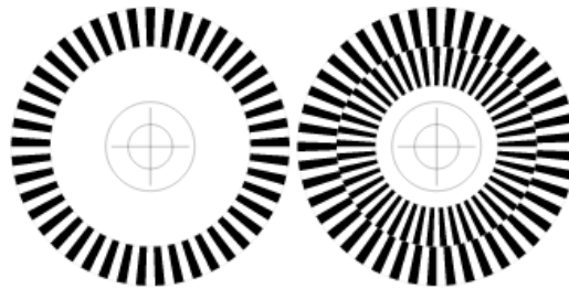
Figure 14 Incremental Encoding Patterns
