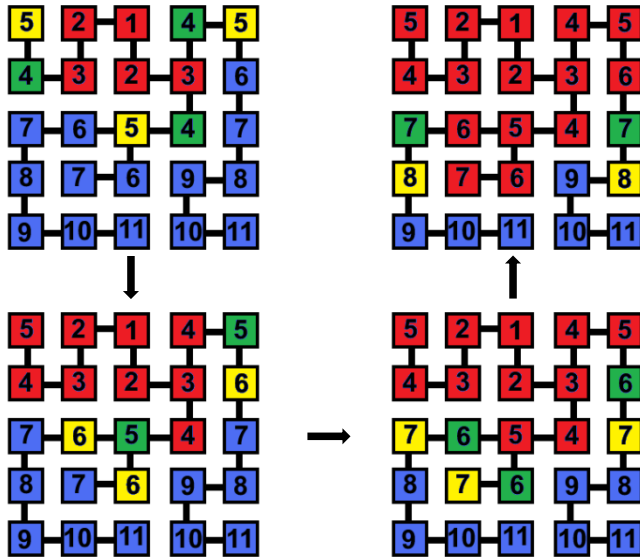
Figure 60 Breadth-First Search Algorithm
