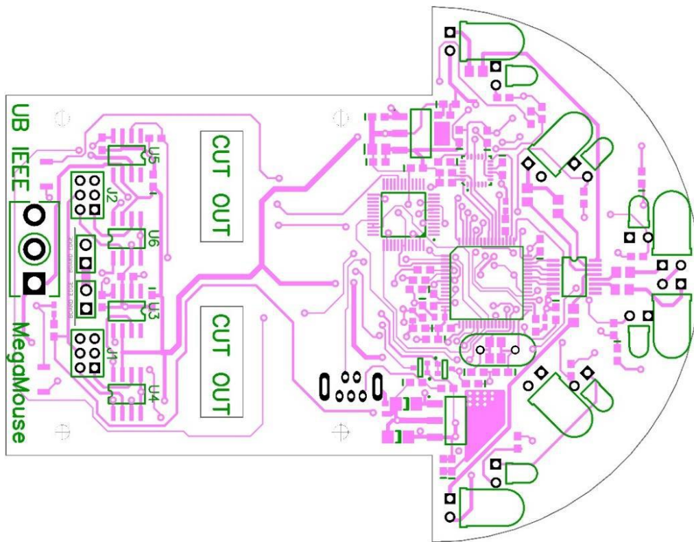
Figure 6: PCB Design of the MicroMouse (permission granted)
