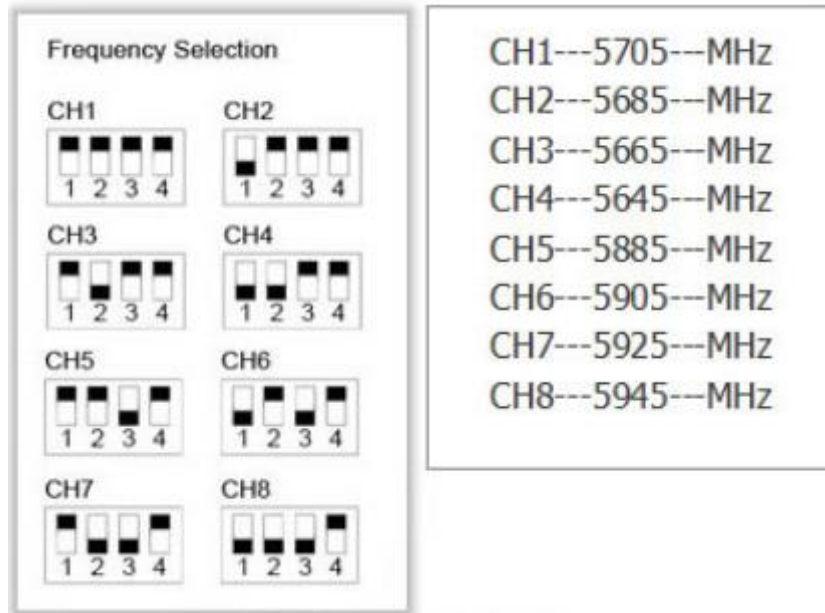
Figure 56 Frequency Selection (permission pending)
