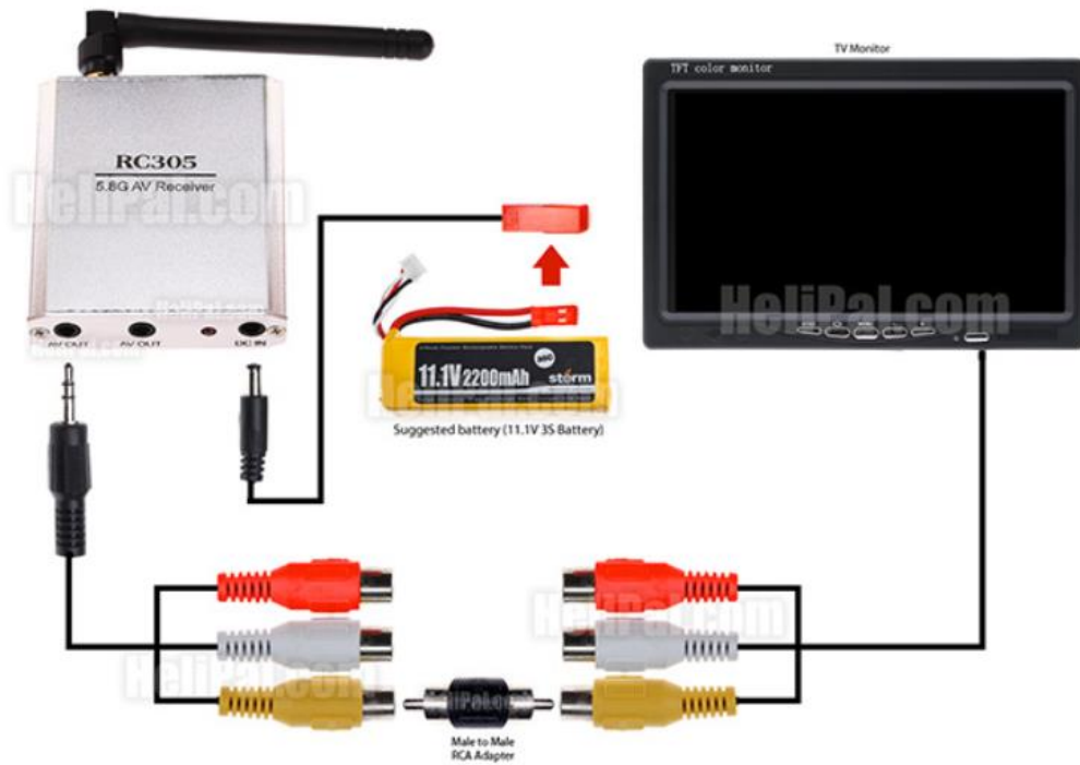
Figure 57 Receiver set up (permission pending)
