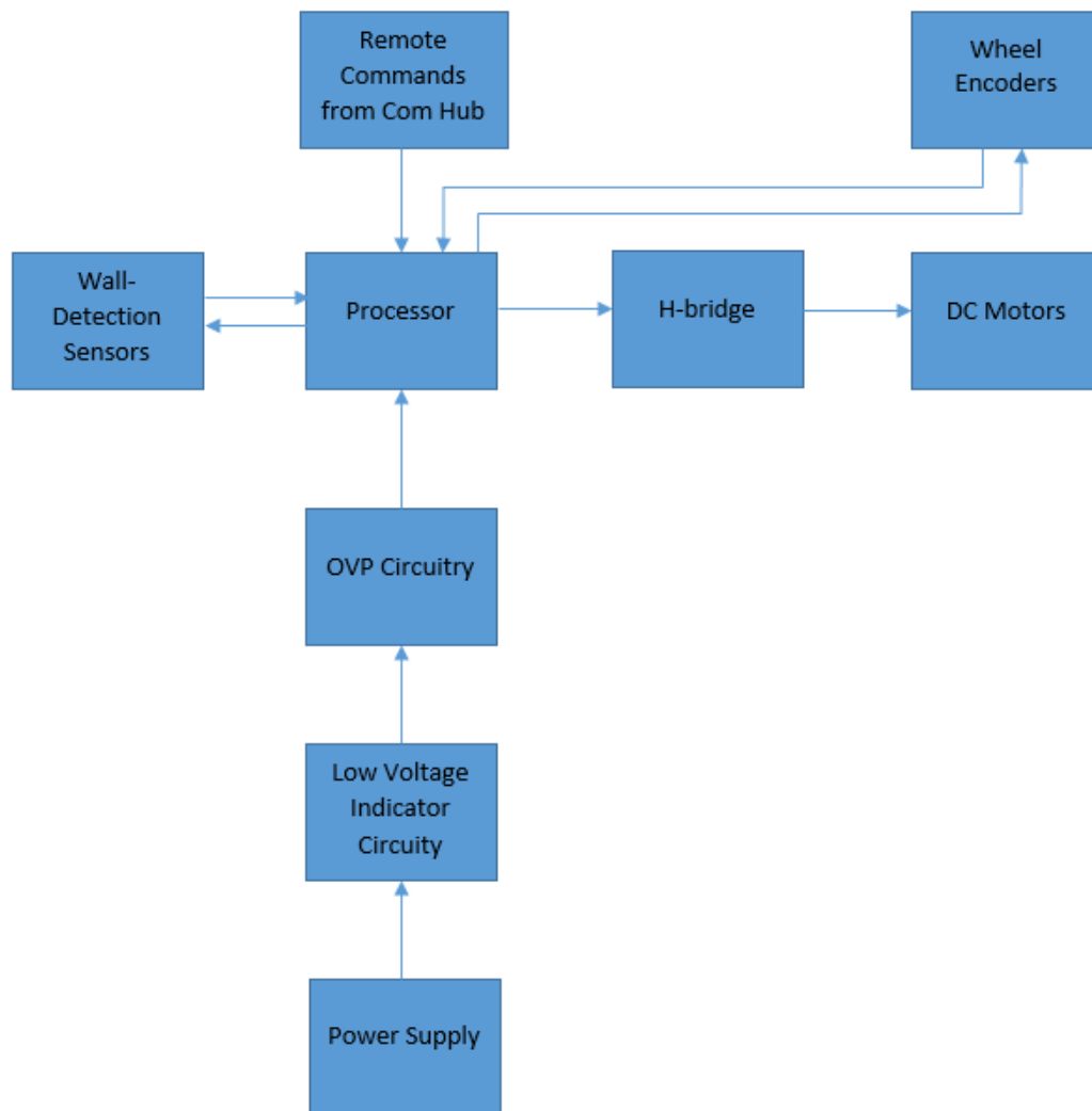
Figure 50 Ground Vehicle Design Flow
