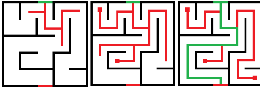
Figure 31 Breadth-First Search
