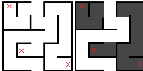
Figure 29 Dead-end filling
