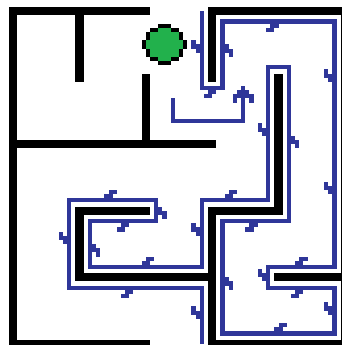
Figure 28 Wall Follower
