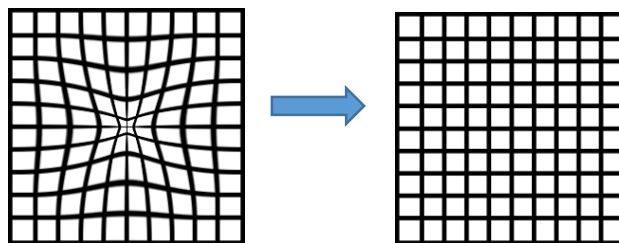
Figure 19 Distortion Correction
