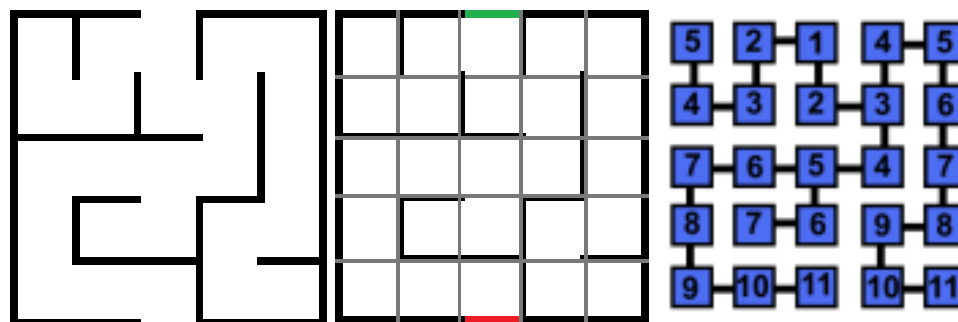
Figure 25 Image conversion
