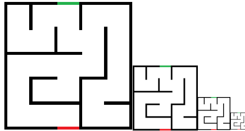
Figure 18 Image Pyramid
