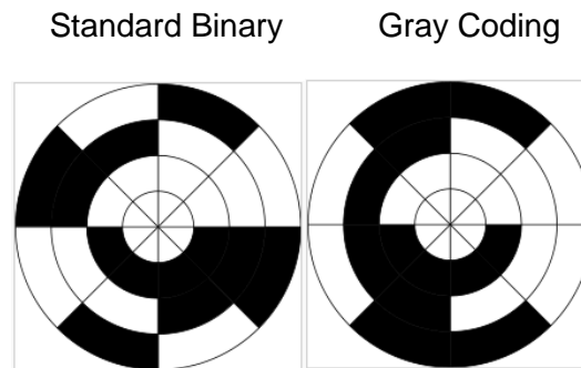
Figure 13 Binary Coding Patterns
