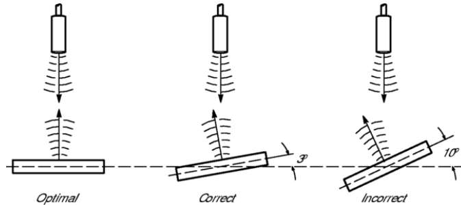
Figure 12 Sensor Orientation (permission pending)
