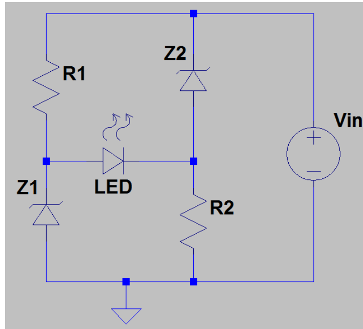
Figure 8: Example Low-Voltage Indicator Circuit
