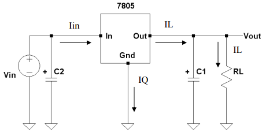
Figure 9: Linear Regulator Circuit (permission pending)
