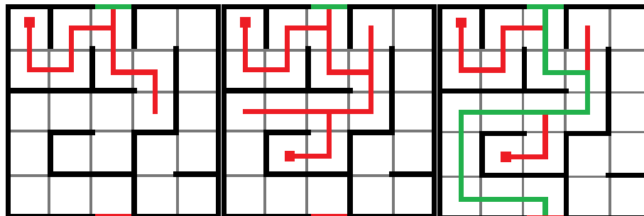
Figure 32 A* Algorithm
