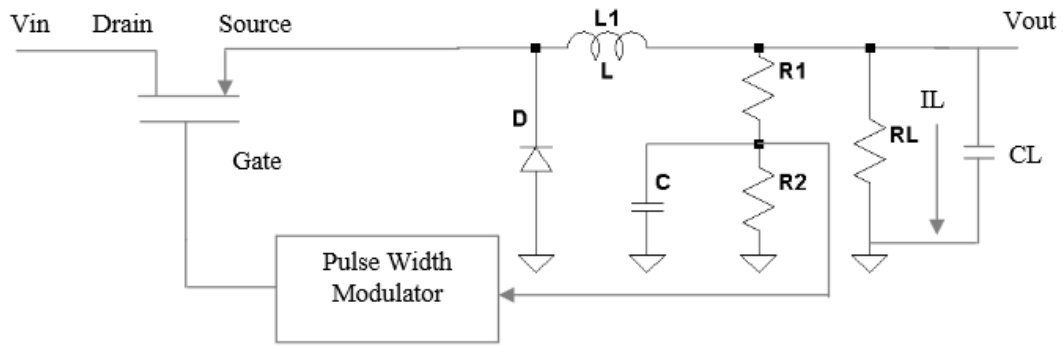
Figure 10: Switching Regulator Circuit (permission pending)
